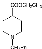
H52374 Ethyl 1-benzylpiperidine-4- carboxylate, 97+% [24228-40-8]
