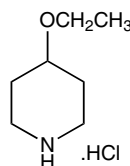
H51028 4-Ethoxypiperidine hydrochloride
