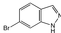
H32623 6-Bromo-1H-indazole, 95% [79762-54-2]
