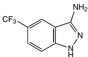
H32995 3-Amino-5-(trifluoromethyl)-1H-indazole, 97% [2250-53-5]
