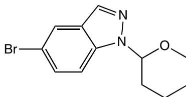
H31755 5-Bromo-1-(2-tetrahydropyranyl)-1H-indazole, 95%
