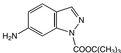
H32010 1-Boc-6-amino-1H-indazole, 97% [219503-81-8]
